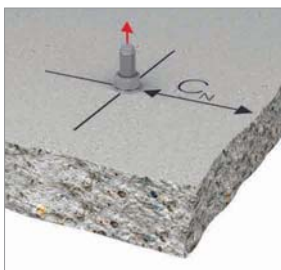
Reduction factor related to the distance c_N of the fixing from the edge, in cases where load is not being applied towards a free edge: f_{c_N}
