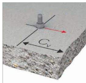
Reduction factor related to the distance c_V of the fixing from the edge, in cases where load is being applied towards a free edge: f_{c_V}
